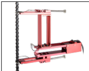
Extensometer
