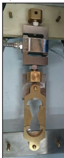
1000N Load Cell with Mould Guide Piece
